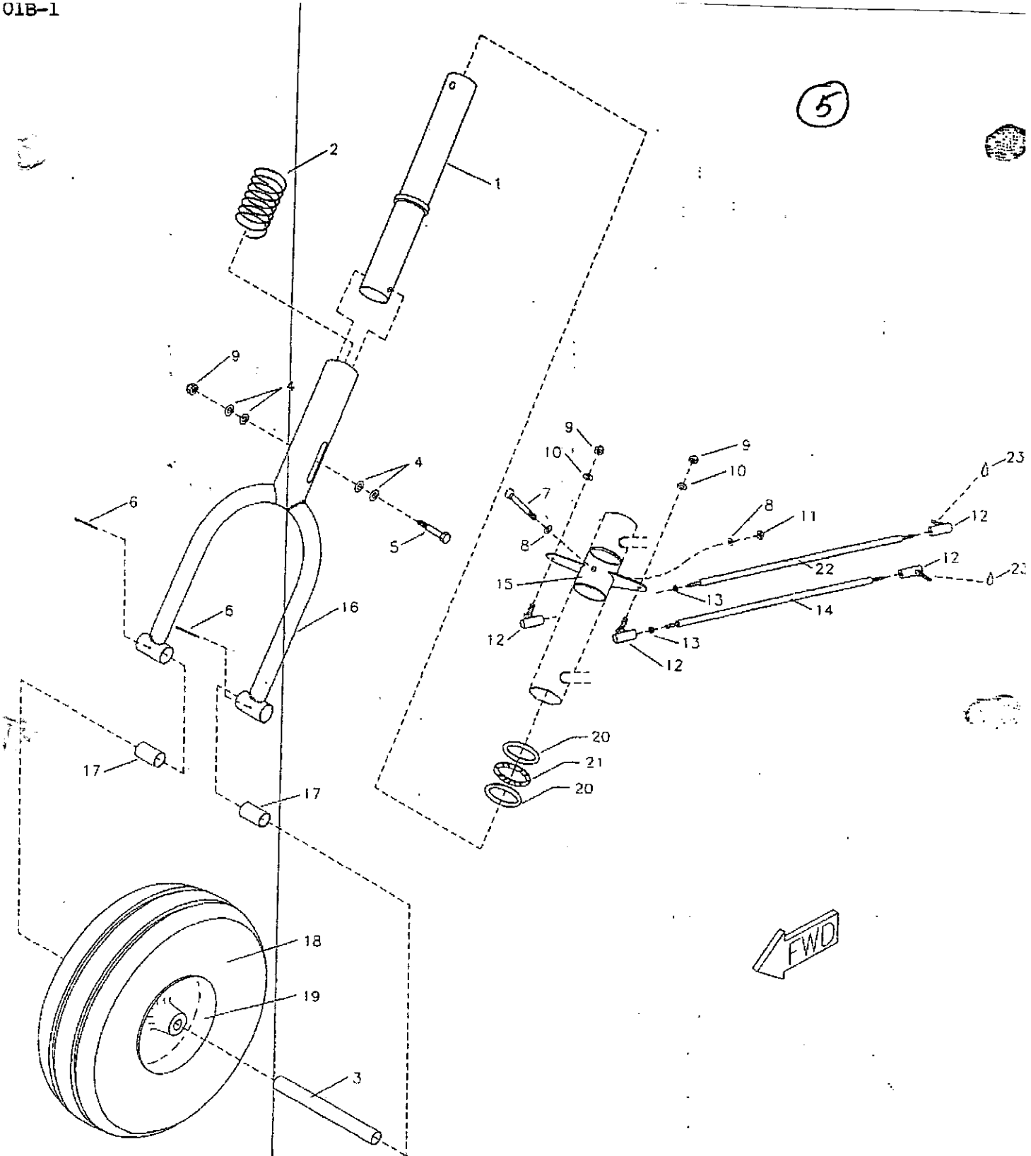
RANS S-12 AIRAILE NOSE GEAR ASSEMBLY
